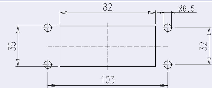
Panel cut out for bulkhead mounting
