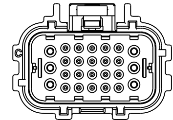
KEY C LVRFC26PCC MATE CONNECTOR P/N: LVRCM26SCRC.
